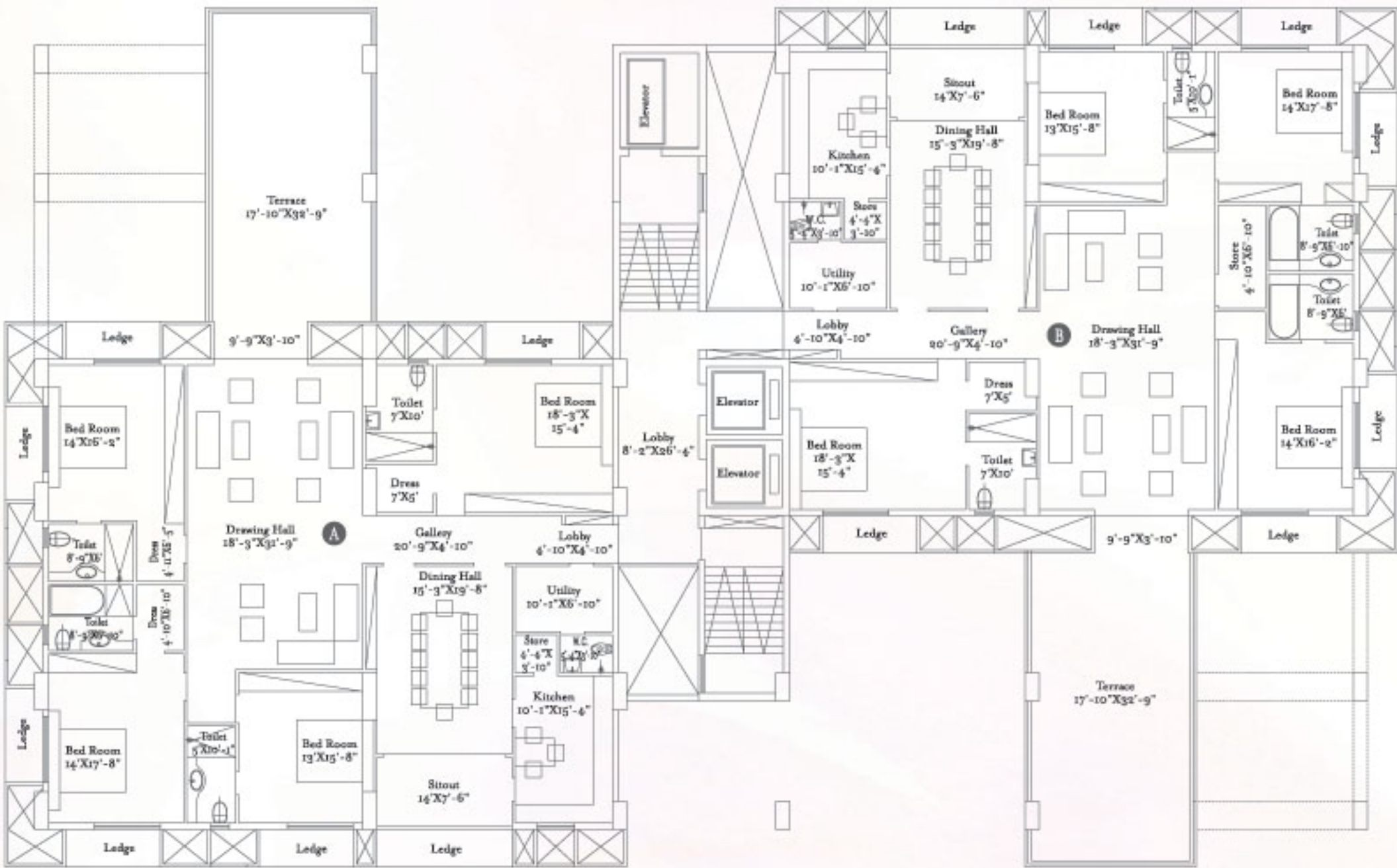
5TH, 8TH, 11TH & 14TH FLOOR PLAN
