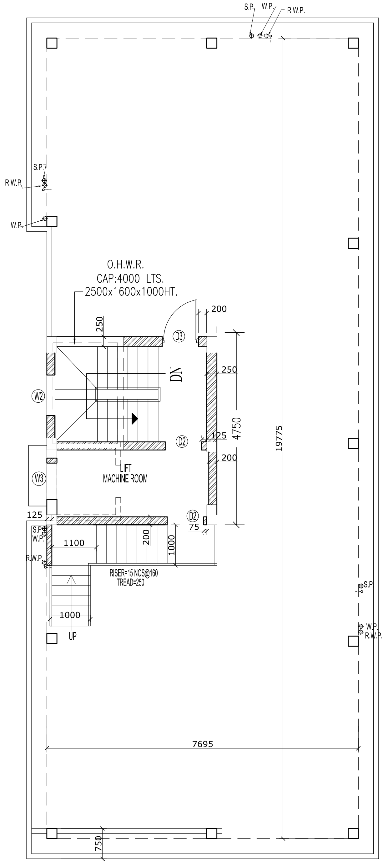
ROOF PLAN
