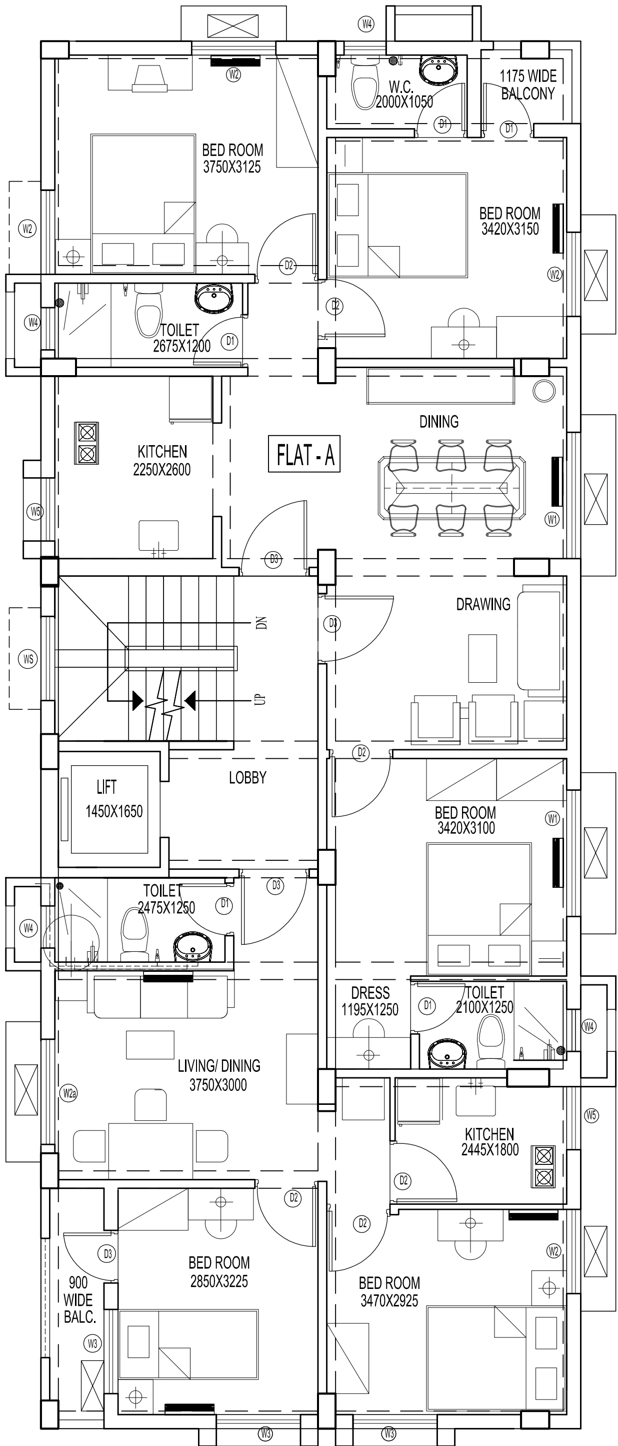
2 ND FLOOR PLAN
